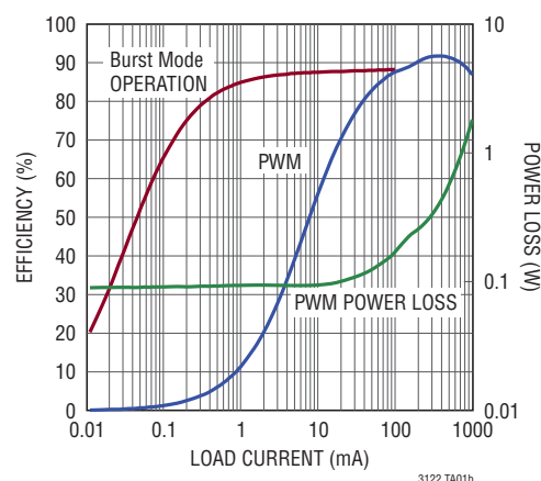
Efficiency Curve
